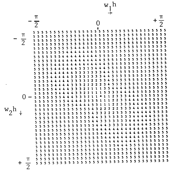
Fig. 2a'. b_1 = \sqrt{2} , b_2 = \sqrt{2} , \bar{\beta} = 2\beta
