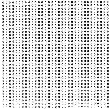
Fig. 2a. b_1 = \sqrt{2} , b_2 = \sqrt{2} , \bar{\beta} = \beta
