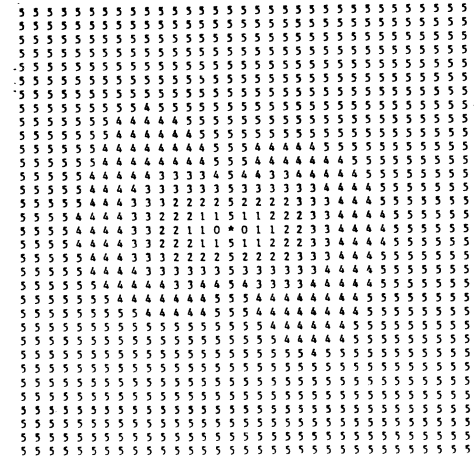
Fig. 2c'. b_1 = 1 , b_2 = 0 , \bar{\beta} = 2\beta
