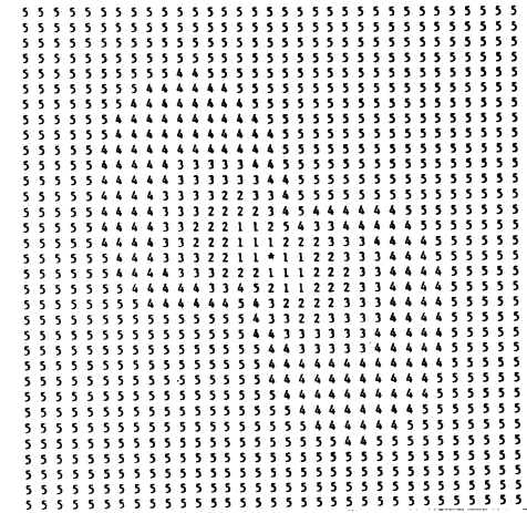
Fig. 2b'. b_1 = \frac{1}{2}\sqrt{3} , b_2 = \frac{1}{2} , \bar{\beta} = 2\beta
